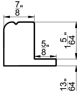
Sill Plate for 1 1/4" Beaded Z and 1 1/2" Bullnose Z Frames
