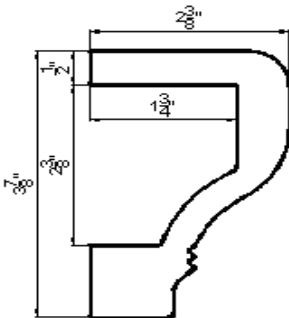
Designer Sill Cap For L Frame
