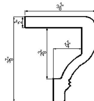
Cap Designer Sill Cap For Z Frame
