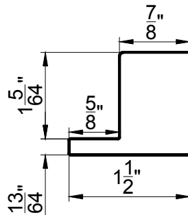
Sill Plate for 1 1/4" Beaded Z and 1 1/2" Bullnose Z Frames
