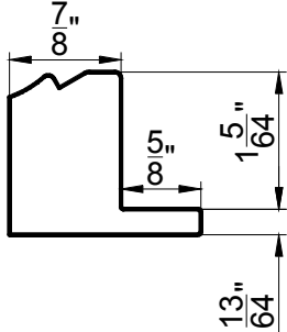
3" Ridge Deco Sill Plate
