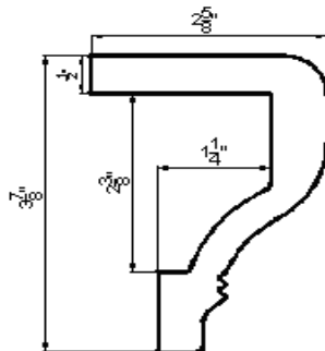
Designer Sill For Deco & Hang Strip
