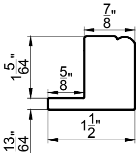
2" Bel Air Z Sill Plate
